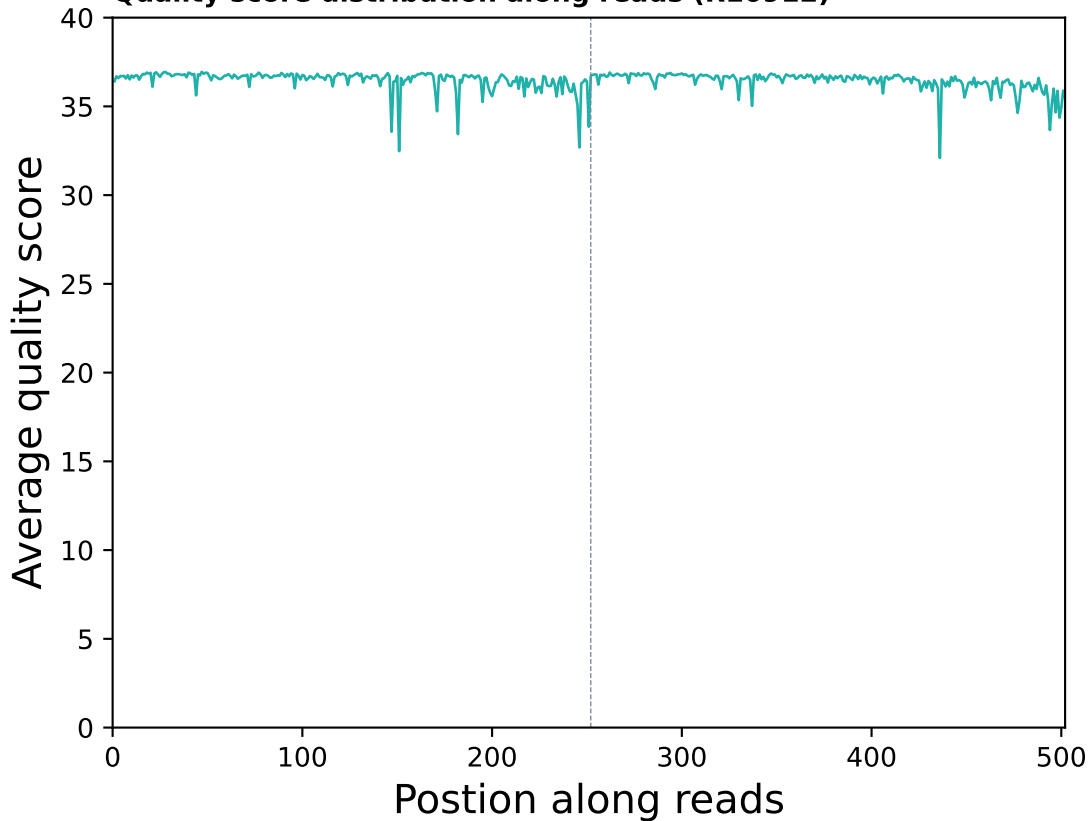
Quality score distribution along reads (R10912)
